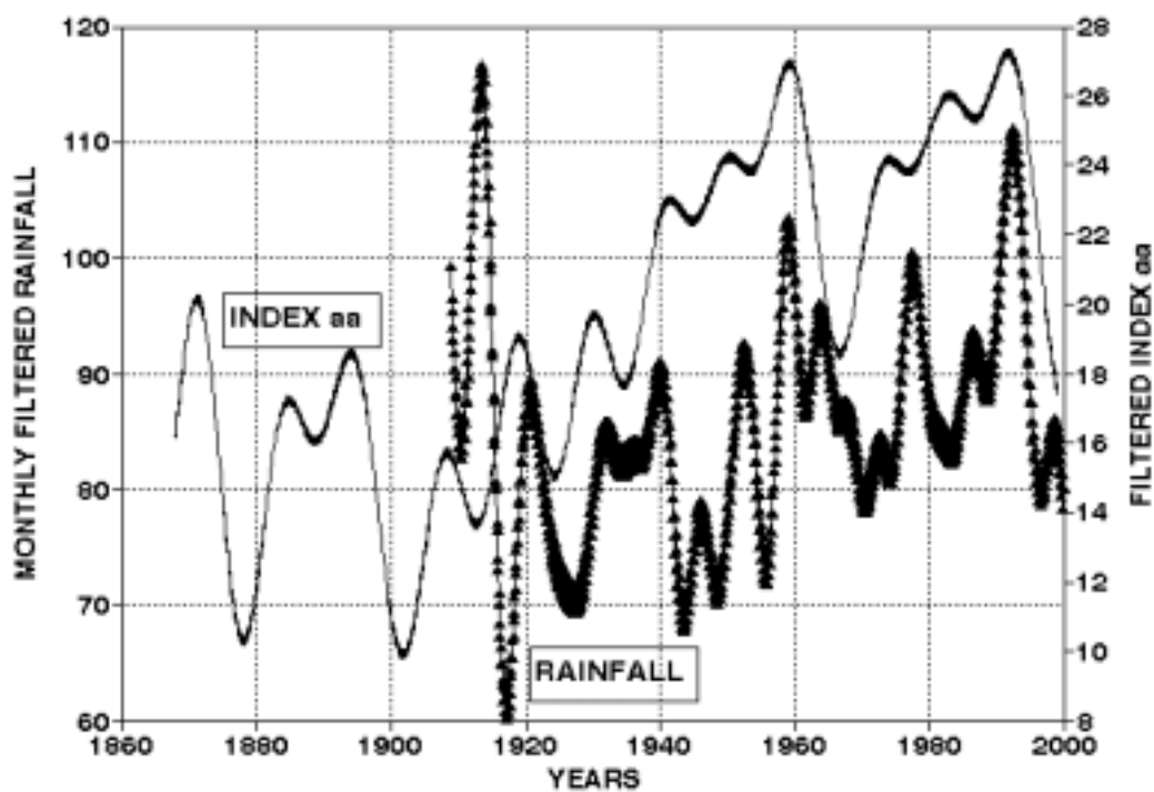
Fig. 5. Rainfall and aa index series.
