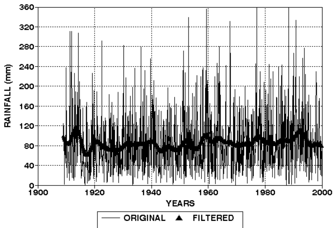
Fig. 4. The original and filtered rainfall serie.
